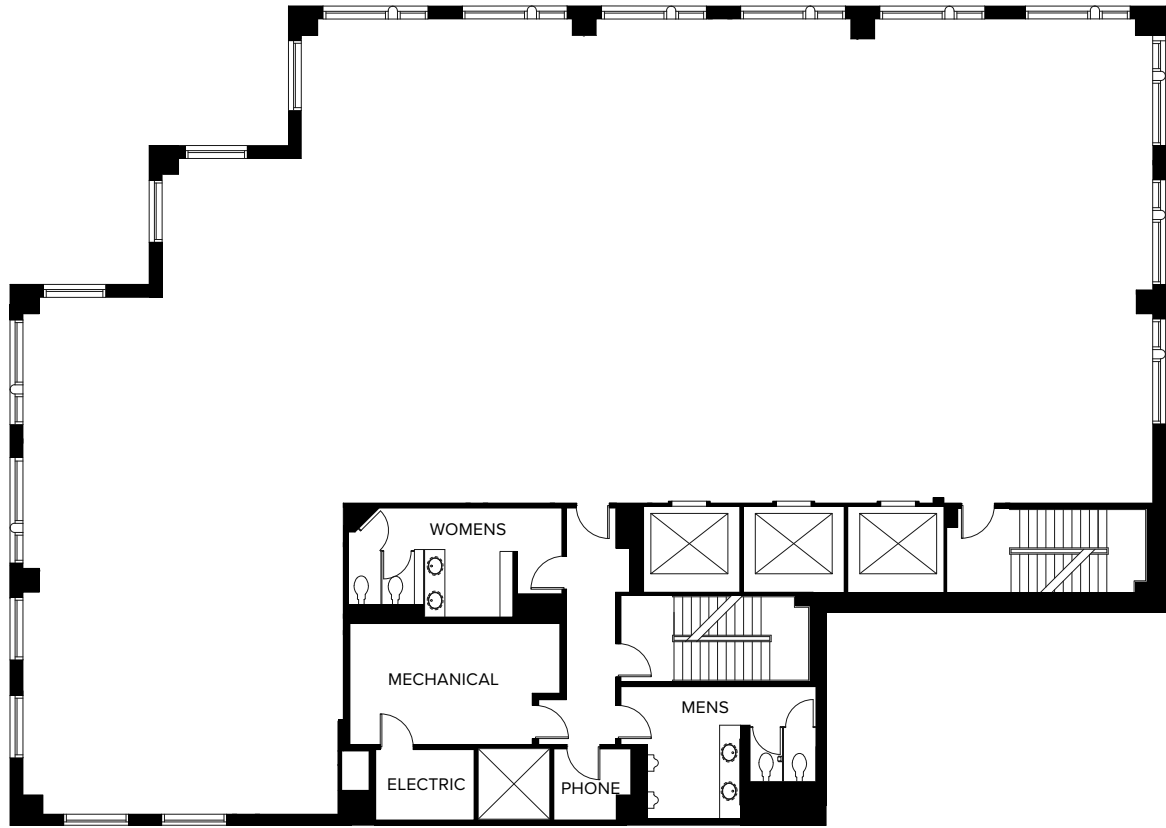
TOWER FLOOR PLAN
